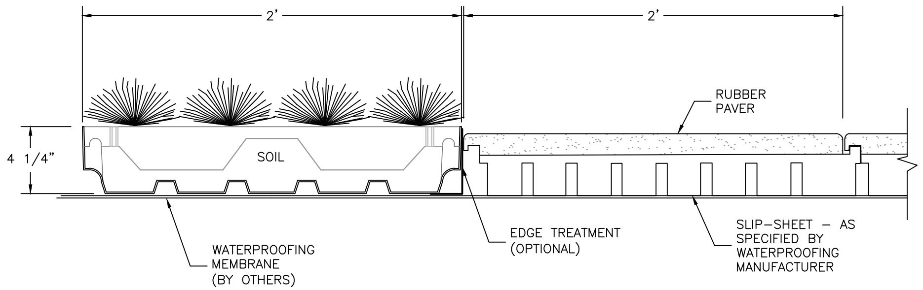
CROSS SECTION
