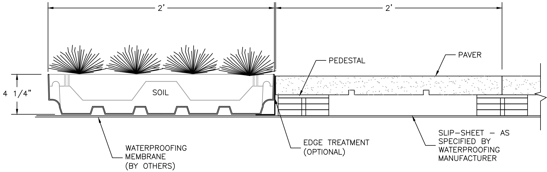
CROSS SECTION
