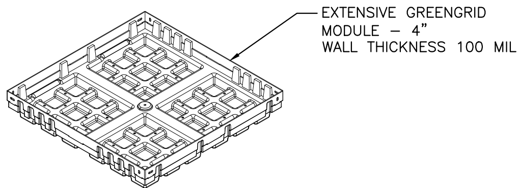
ISOMETRIC VIEW
