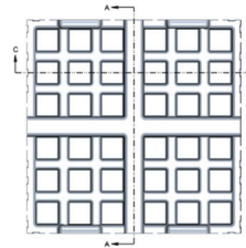
Top View 4" Tray
