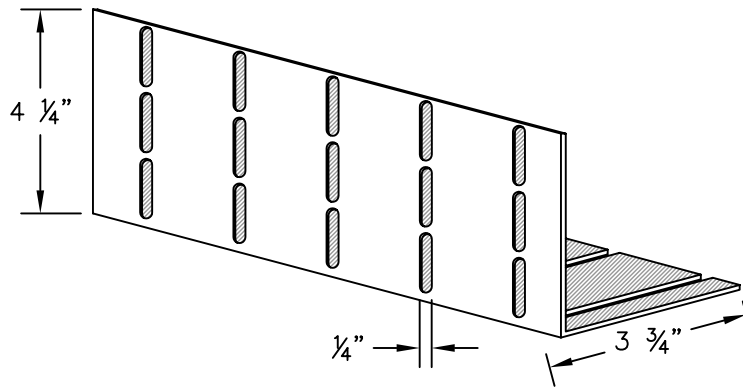
ISOMETRIC VIEW
